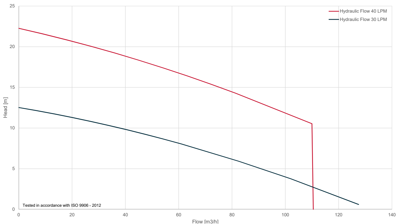
4" Submersible Pump
